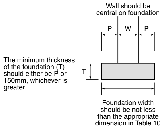
Diagram 24 Foundation dimensions
