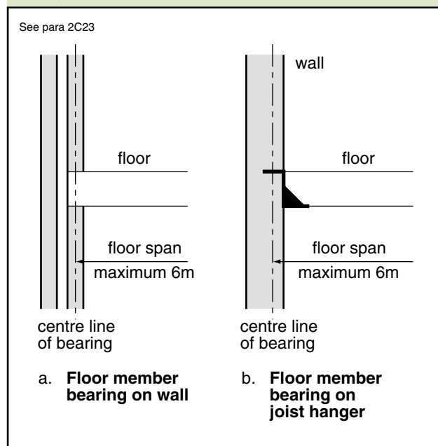
Diagram 11 Maximum span of floors
