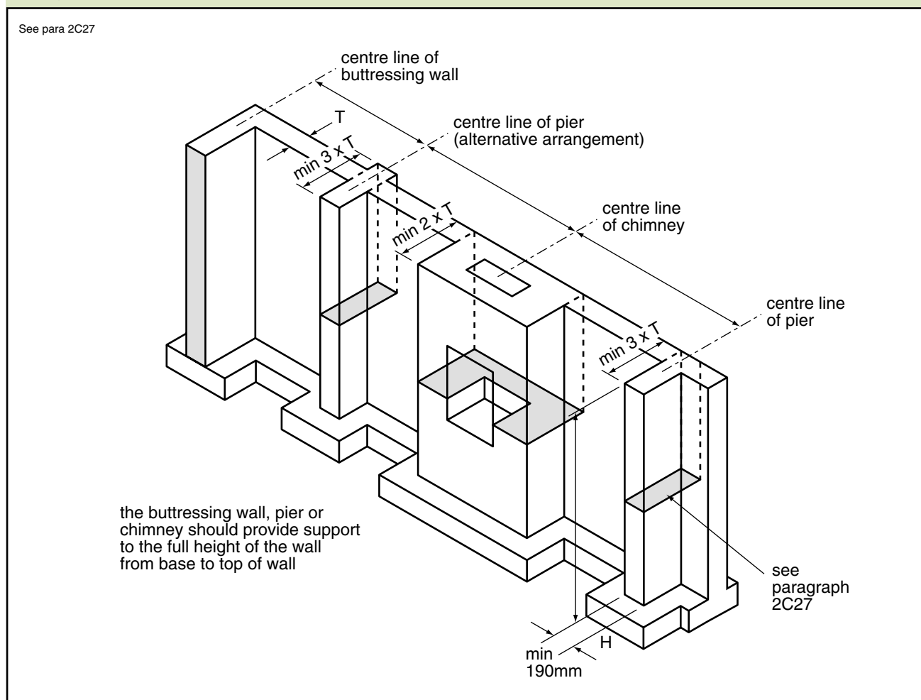
Diagram 14 Buttressing
