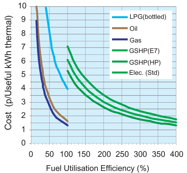
Figure 6: Domestic fuel costs* versus fuel utilisation efficiency
