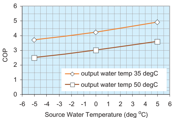
Figure 5: Coefficients of performance of typical small GSHP's
