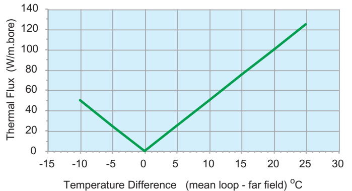
Figure 4: Thermal flux from a single U-tube closed-loop borehole
