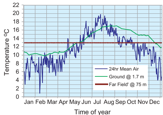
Figure 3: Air and ground temperatures, Falmouth 1994 (Source: Geoscience Limited)
