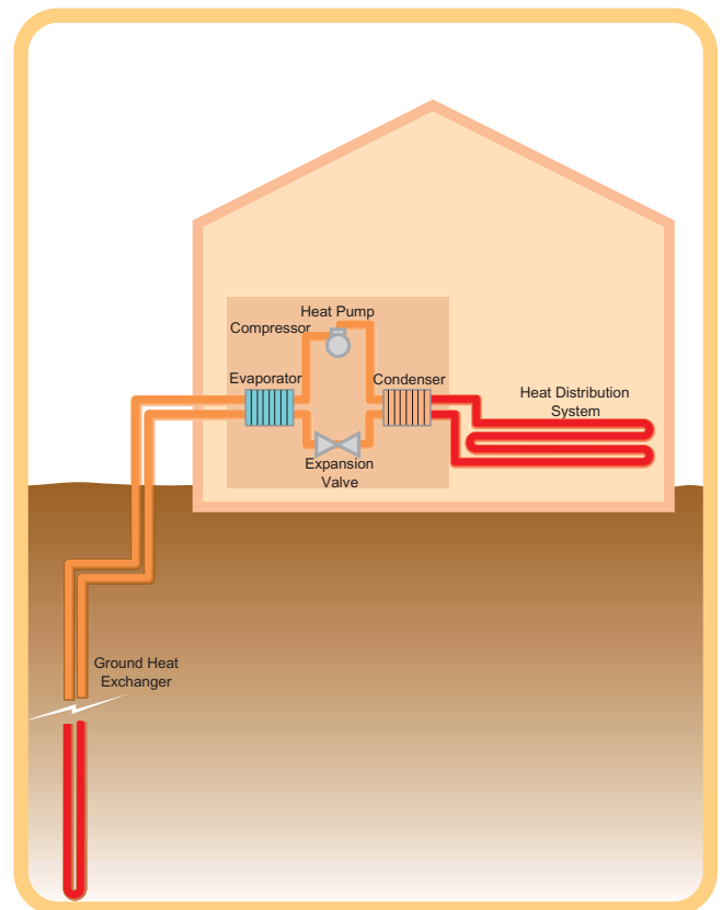
Figure 1: A typical GSHP system
