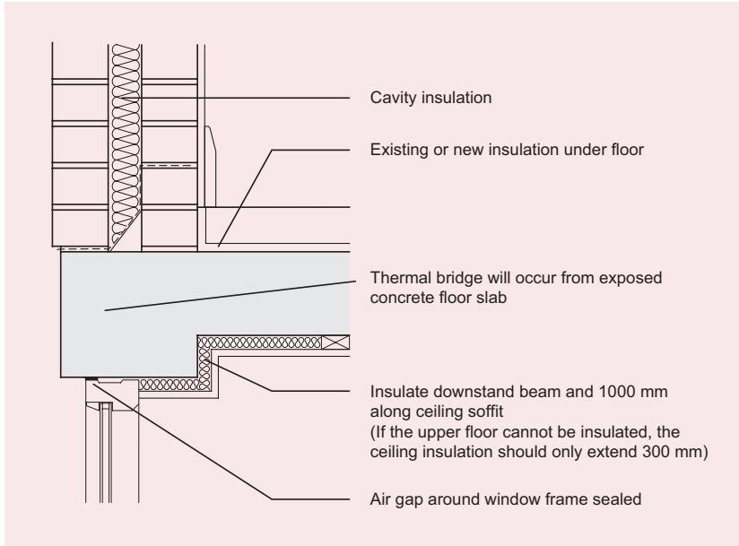
Figure 4 Insulating thermal bridge at floor slab
