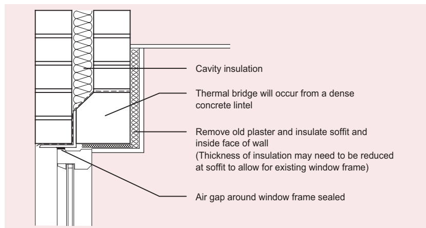
Figure 3 Insulating thermal bridge at lintel
