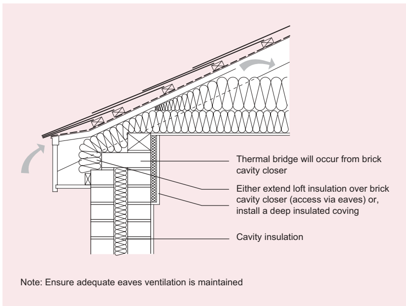
Figure 5 Insulating thermal bridge at eaves
