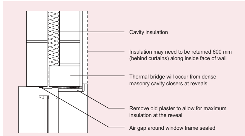
Figure 2 Insulating thermal bridge at reveal
