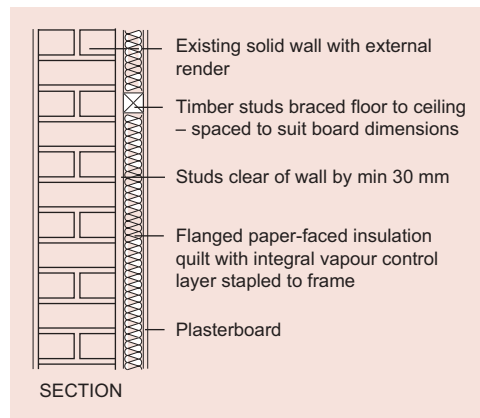
Figure 4 Insulation fitted to battens
