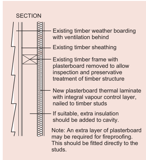
Figure 2 Timber framed external wall with plasterboard laminate
