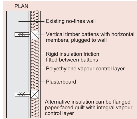
Figure 3 Timber stud frame inside solid no fines wall
