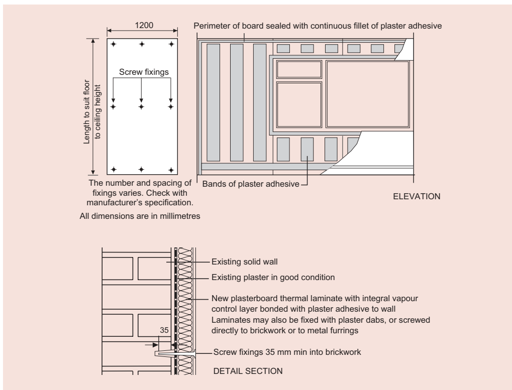
Figure 1 Plasterboard thermal laminate
