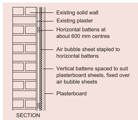
Figure 5 Polyethylene air bubble sheet
