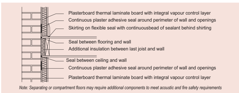
Figure 6 Timber stud frame in existing flats
